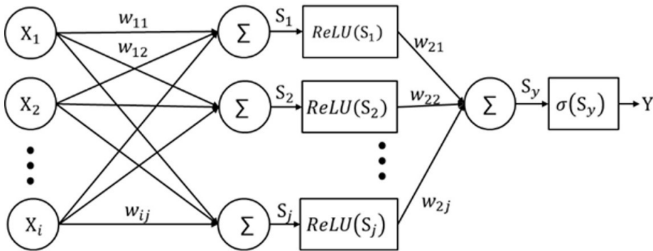
Figure 6. Neural network architecture for font classification
